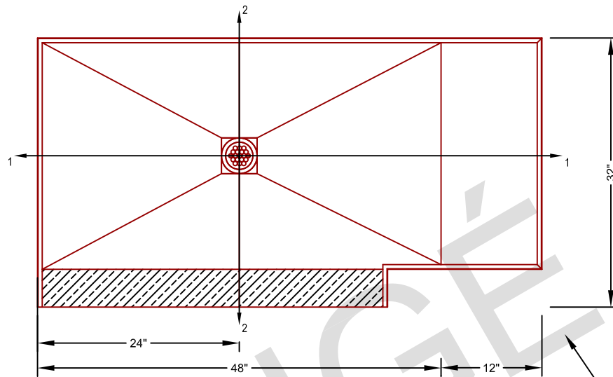
ANGÉ TILE-EZ SHOWER PRIVACY WALL BENCH DESIGN
