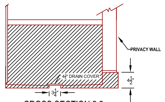
CROSS SECTION 2.2
