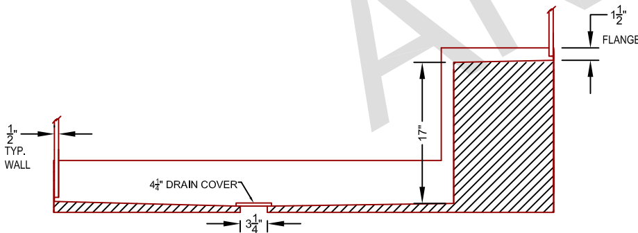
CROSS SECTION 1.1
