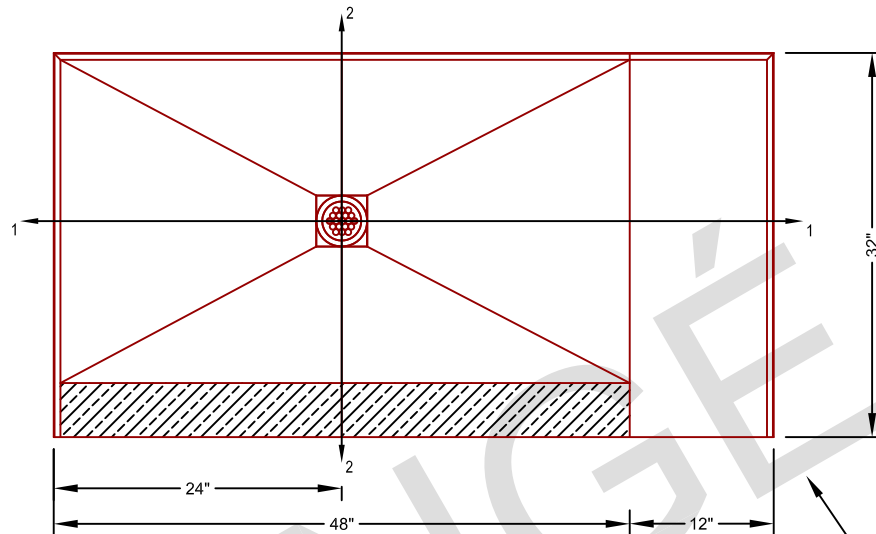
ANGÉ TILE-EZ SHOWER EURO BENCH DESIGN
