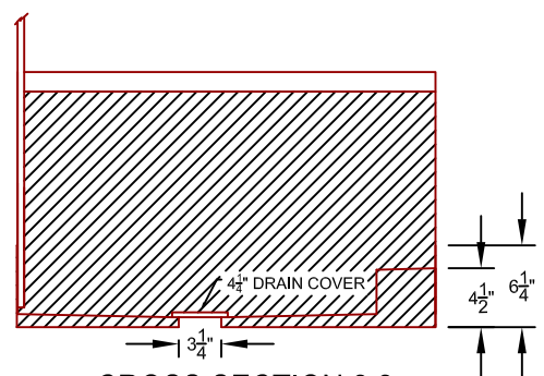
CROSS SECTION 2.2
