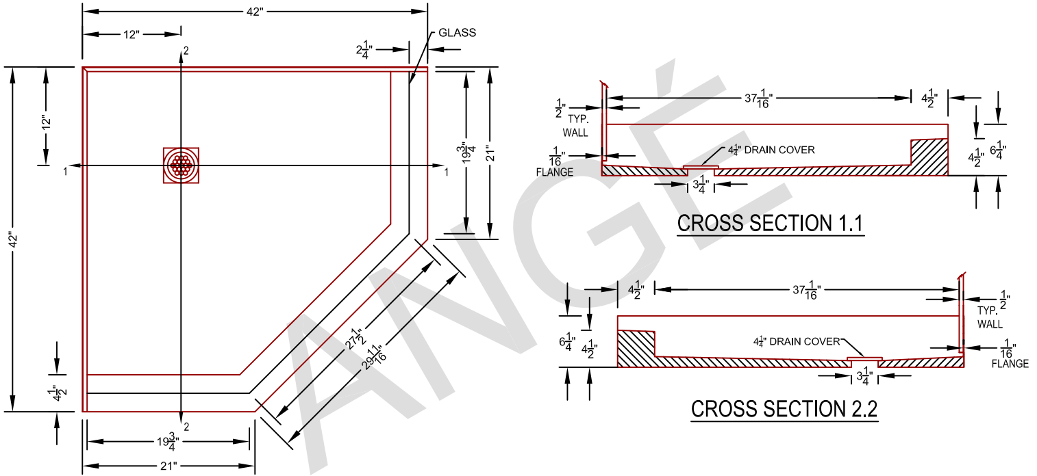
ANGÉ TILE-EZ SHOWER PAN WITH CURB
