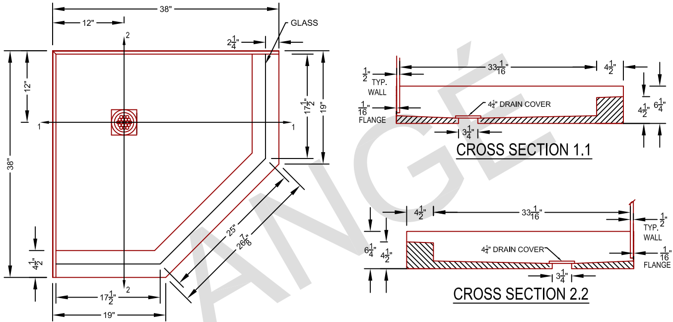
ANGÉ TILE-EZ SHOWER PAN WITH CURB
