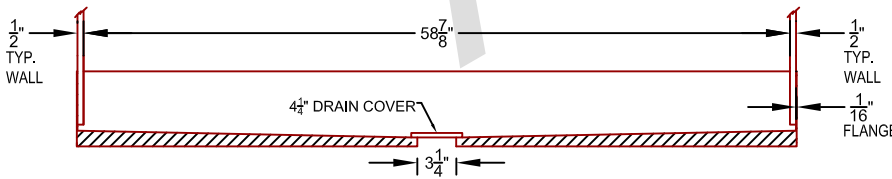
CROSS SECTION 1.1
