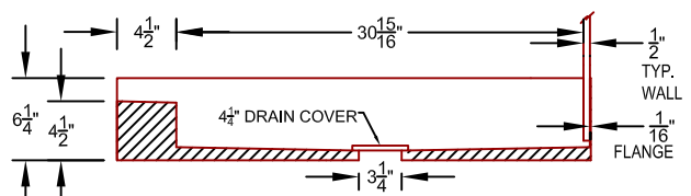
CROSS SECTION 2.2
