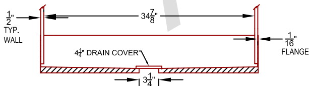
CROSS SECTION 1.1
