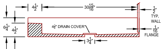
CROSS SECTION 2.2
