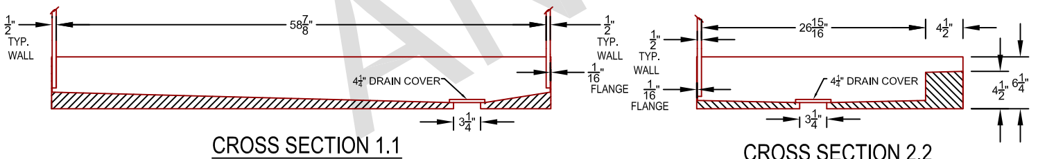
ANGÉ TILE-EZ SHOWER PAN WITH CURB
