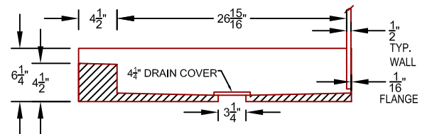
CROSS SECTION 2.2
