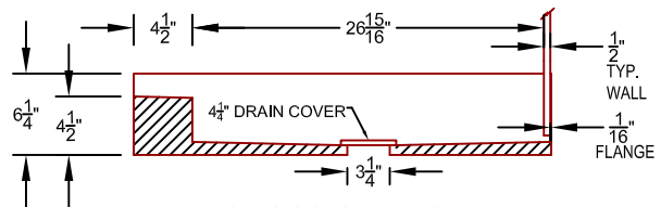
CROSS SECTION 2.2
