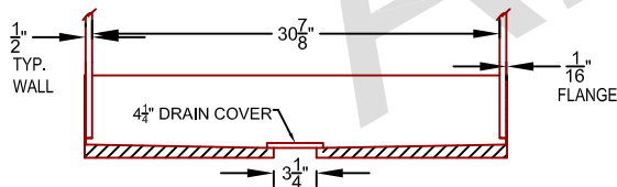
CROSS SECTION 1.1
