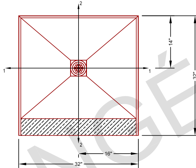
ANGÉ TILE-EZ SHOWER PAN WITH CURB
