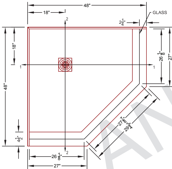
ANGÉ TILE-EZ SHOWER PAN WITH CURB
