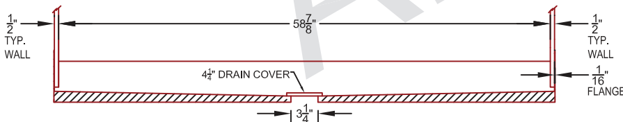
CROSS SECTION 1.1
