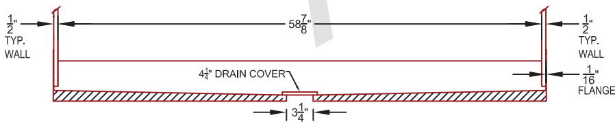
CROSS SECTION 1.1
