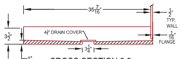
CROSS SECTION 2.2
