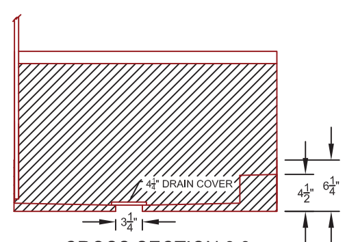
CROSS SECTION 2.2
