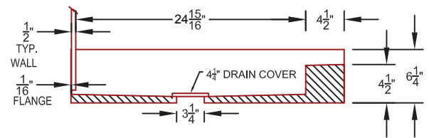
CROSS SECTION 2.2
