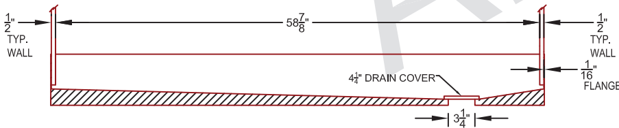
CROSS SECTION 1.1
