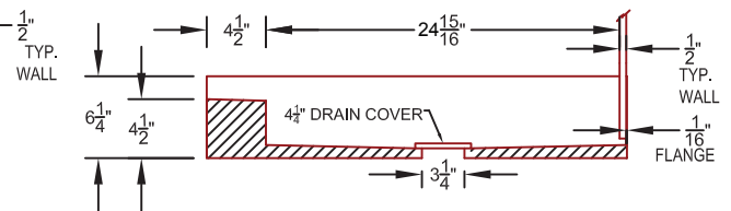
CROSS SECTION 2.2
