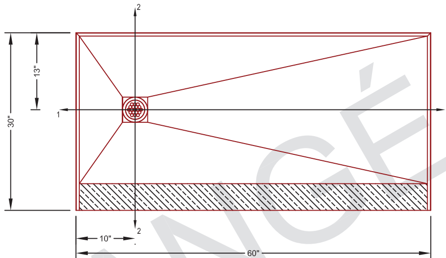
ANGÉ TILE-EZ SHOWER PAN WITH CURB
