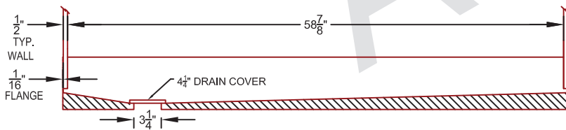
CROSS SECTION 1.1
