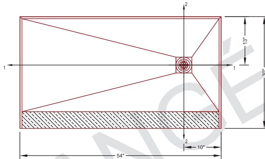
ANGÉ TILE-EZ SHOWER PAN WITH CURB
