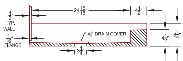
CROSS SECTION 2.2
