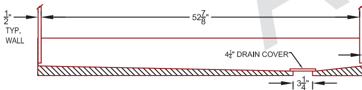
CROSS SECTION 1.1
