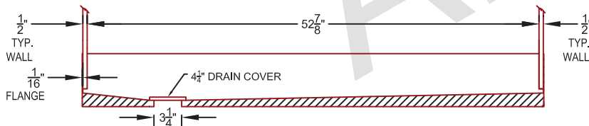
CROSS SECTION 1.1
