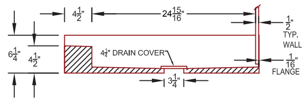
CROSS SECTION 2.2
